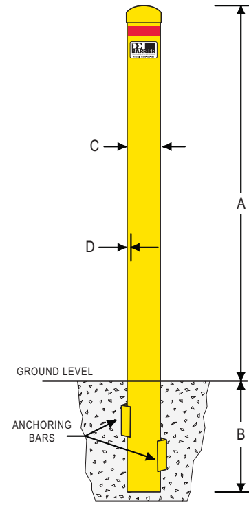
BELOW-GROUND MODEL
